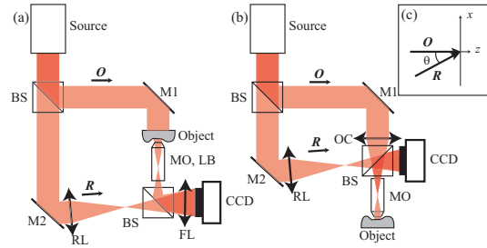
Fig. 1. Digital holographic microscope, (a) transmission and (b) reflection setups. O object wave; R reference wave; BS beam splitter; M1, M2 mirrors; MO microscope objective, RL lens in the reference wave, OC condenser in the object wave, FL field lens and LB lens ball.(c) Detail of the off-axis geometry.
